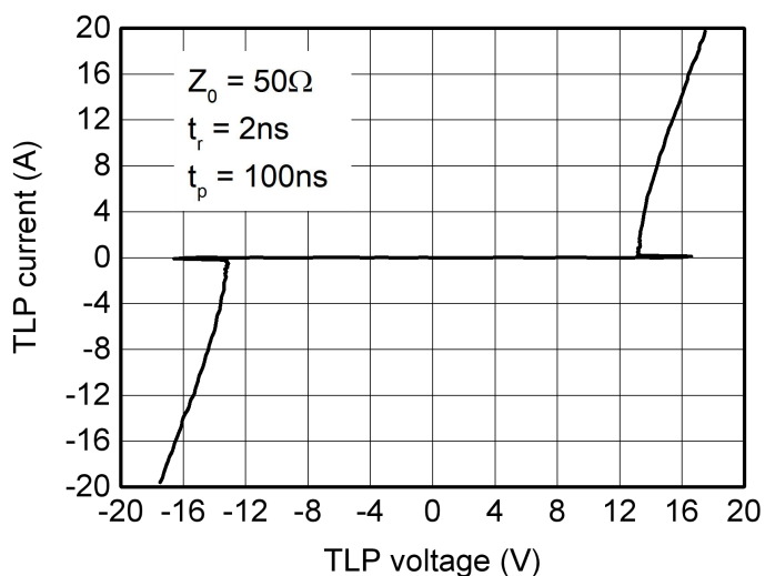
TLP Measurement
